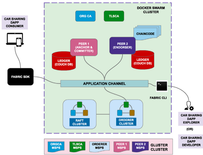
Fig. 8. TIC (trust and integration controller) hyperledger fabric service configuration for a sample car-sharing organization.
